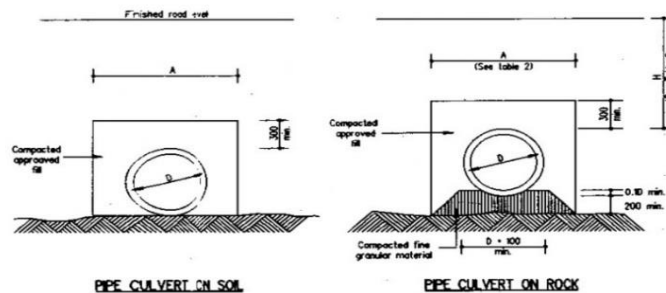
CLASS C BEDDING (EMBANKMENT CONDITION)
