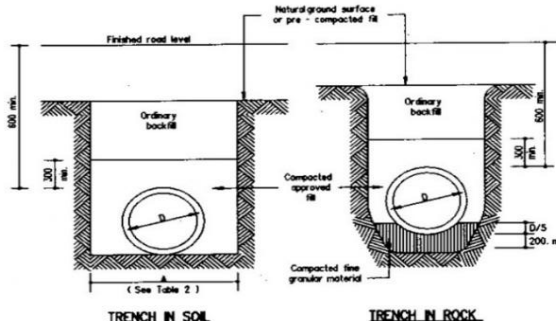
CLASS C BEDDING (TRENCH CONDITION)
