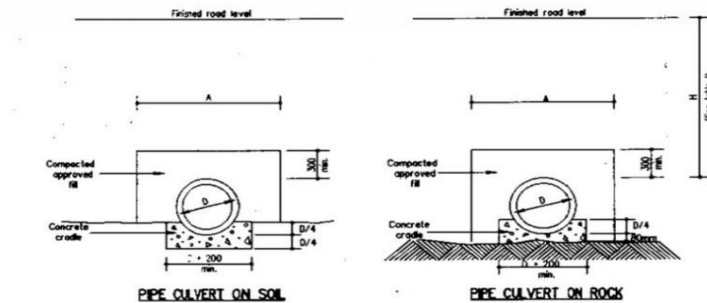
CLASS A BEDDING (EMBANKMENT CONDITION)
