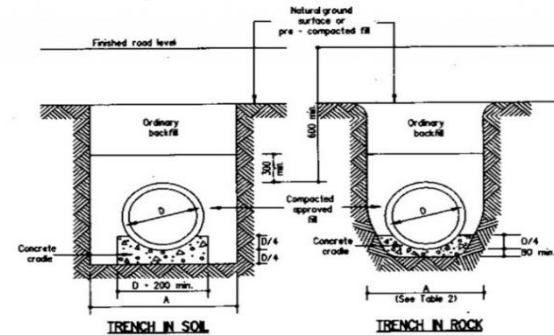
CLASS A BEDDING (TRENCH CONDITION)
